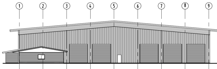
North Elevation
