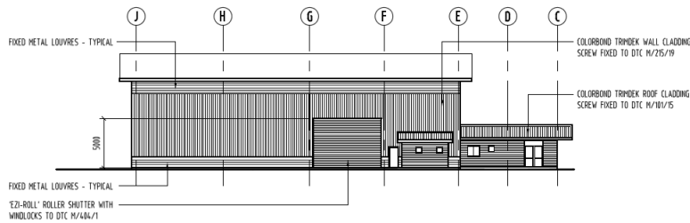
East Elevation
